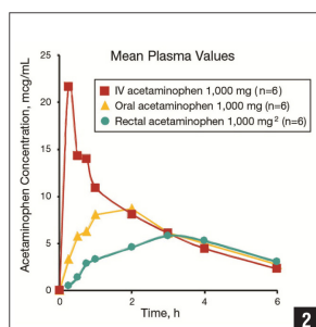
Figure 2: Mean acetaminophen plasma concentration over time in 6 test subjects after intravenous (IV), oral and rectal administration of 1000 mg. (Reprinted with permission from Singla NK, Parulan C, Samson R, et al. Plasma and cerebrospinal fluid pharmacokinetic parameters after single-dose administration of intravenous, oral or rectal acetaminophen. Pain Pract. 2012; 12:523–532.)
